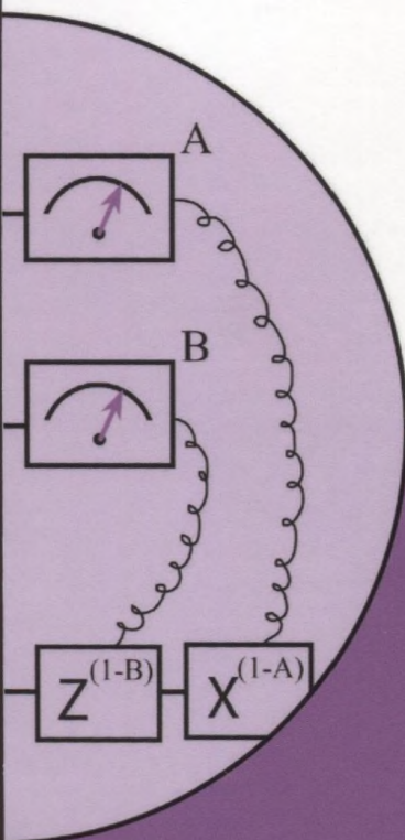
Cover image: A quantum circuit for teleportation (cf. Fig. 6.24)
